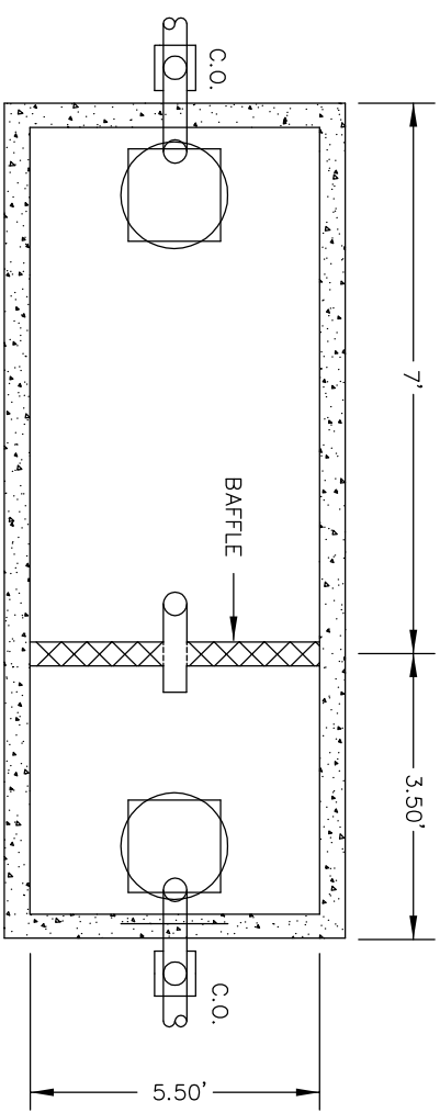
TOP VIEW
